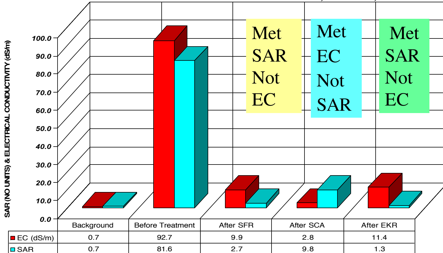
REDUCTION OF SODIUM ABSORPTION RATIO AND ELECTRICAL CONDUCTIVITY IN SURFACE SOILS, AFTER SFR, SCA & EKR TREATMENTS 22-X ROAD MAINTENANCE YARD AND SALT STORAGE SITE, CALGARY, ALBERTA
