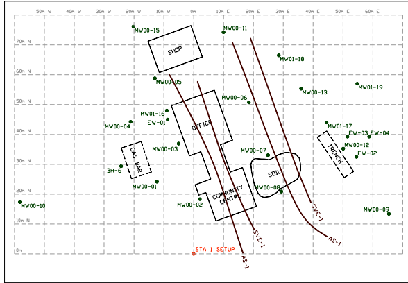
Figure 5. Horizontal Well Location Map
