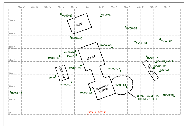
Figure 2. Site Plan
